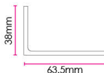
TM 4709 Top Angle Bar *4 (Thickness 3mm)
