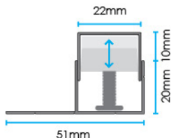
Top Profile, Adjustable Bar & DIY Nuts
