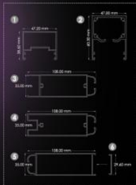
FRAME PROFILE
