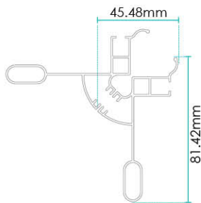
Assembly Corner
