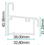
Bottom Track
