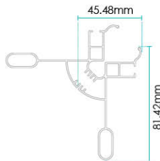
Assembly Corner
