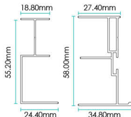
Vertical Frame
