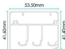
Top Track
