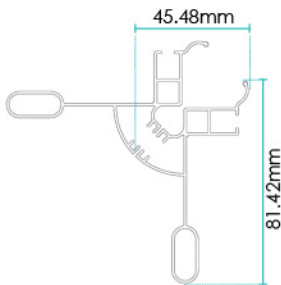
Assembly Corner
