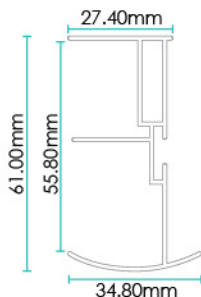
Vertical Frame
