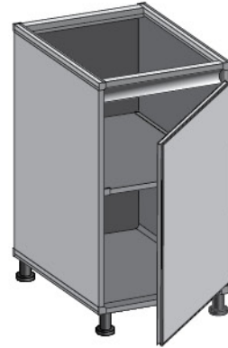
1 1 Door 2301D (Full) / 2301C (Semi)
