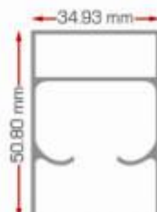
Top Track
