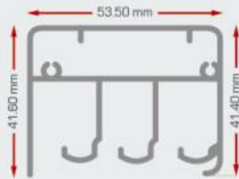
Top Track
