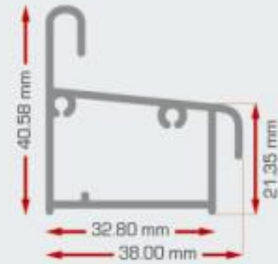
Bottom Track
